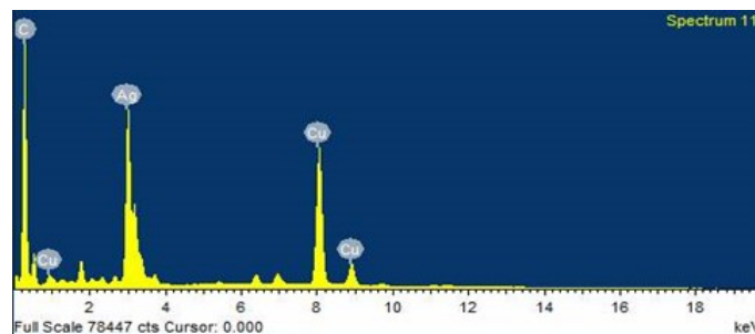
Figure 4. 4: Energy Dispersive Spectroscopy of Conjugated AgNPs
