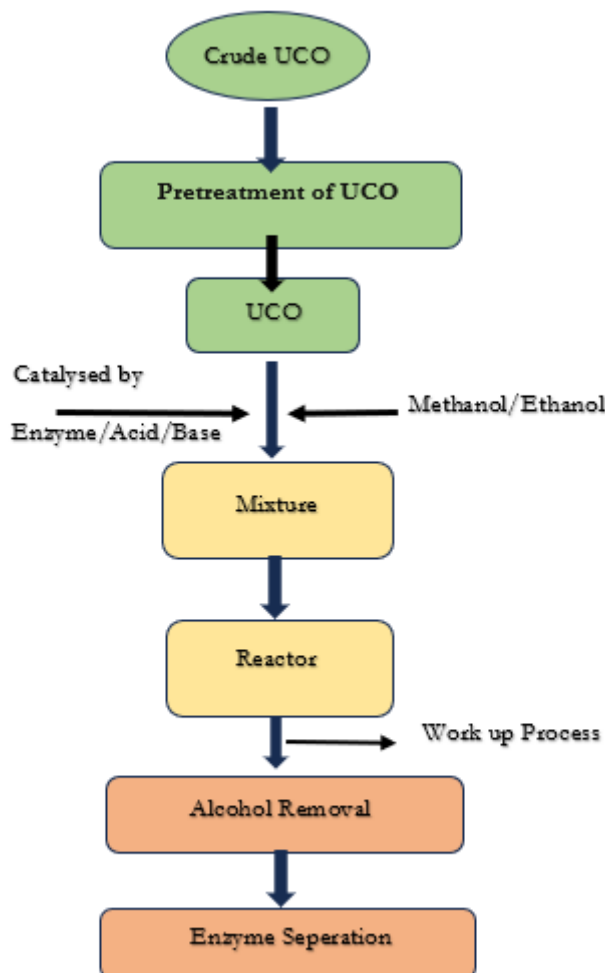
Figure 2: Enzymatic technique for producing biodiesel 55,56,57
