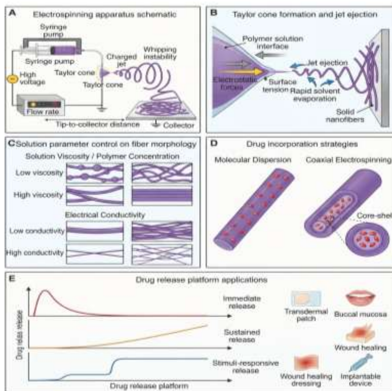
Figure 4. Electrospinning Fiber Formation
