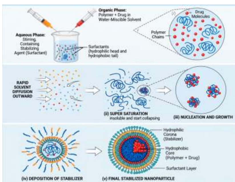
Figure 1. Nanoprecipitation Mechanism
