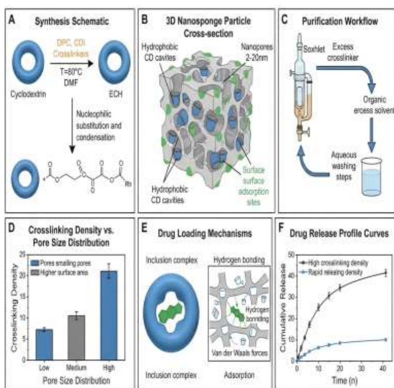
Figure 3. Cyclodextrin Nanosponge Crosslinking Chemistry
