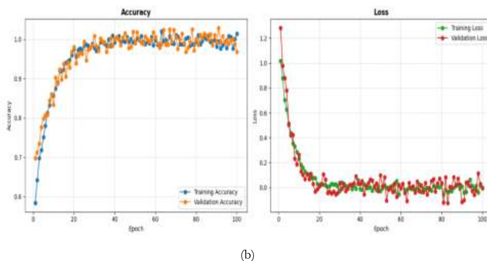
Fig 8. The training and validation/test a) accuracy and b) loss of DMI-Net hybrid model.
