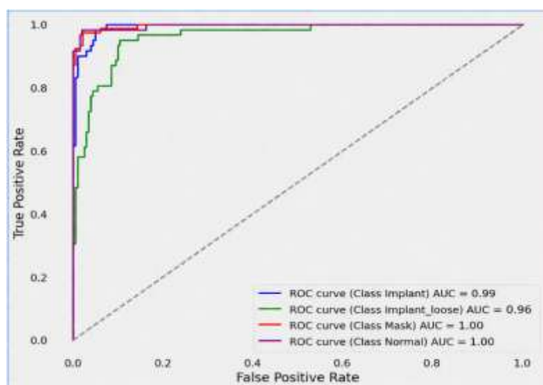
Fig 10. The AUC-ROC curve of the DMI-Net hybrid model.
