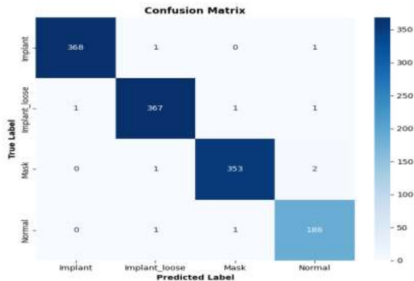
Fig 7: Confusion matrix of DMI-Net hybrid mode.
