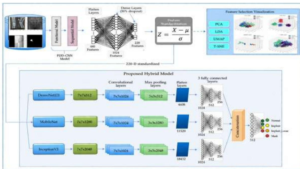
Fig 5: Proposed hybrid DMI-Net architecture integrated with PD-CNN for implant prediction
