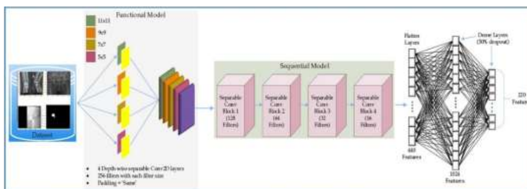
Fig 4: Architecture of the proposed lightweight PD-CNN network for multiscale feature extraction
