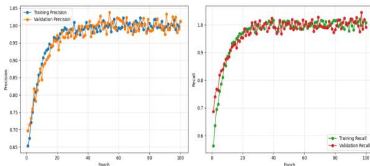
Fig 9. The training and validation/test a) precision and b) recall of the DMI-Net hybrid mode
