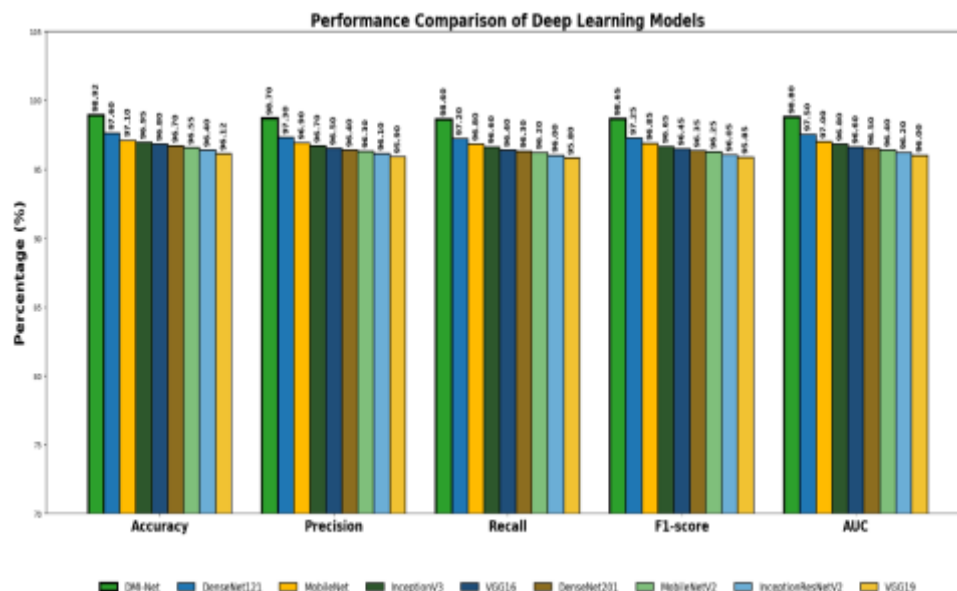
Fig 6: Performance comparison of DL Models
