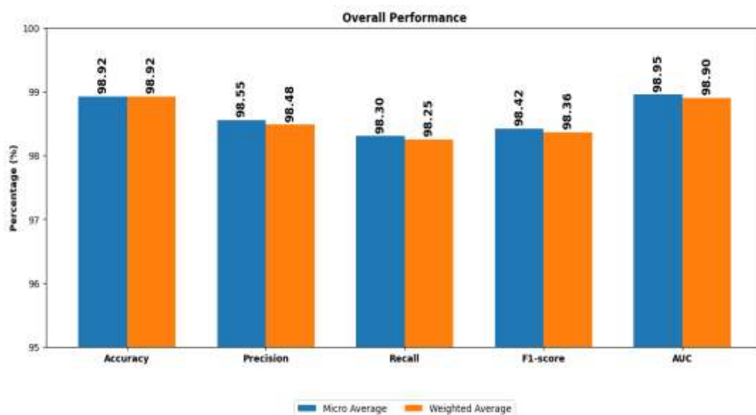
Fig 13. Micro and weight average of all the metrics for the DMI-Net hybrid model
