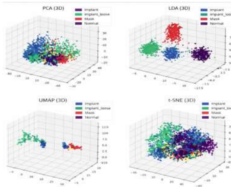
Fig 11. Three-dimensional visualization of the feature embeddings generated by the proposed DMI-Net using four dimensionality-reduction and manifold-projection techniques: PCA, LDA, UMAP, and t-SNE
