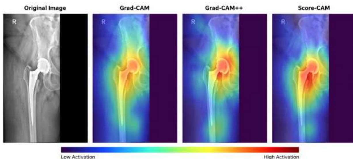
Fig 15: Activation heatmaps generated using Gradient-Weighted Class Activation Mapping (Grad-CAM), Grad-CAM++, and Score-CAM
