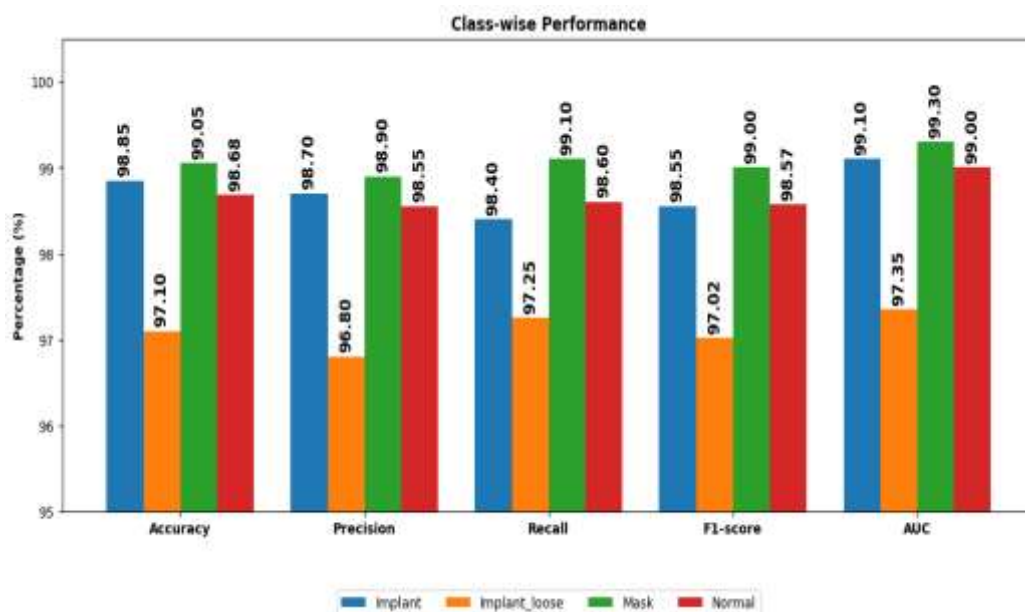
Fig 12. Class-wise performance metrics of DMI-Net hybrid model
