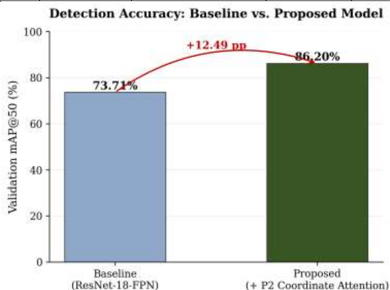
Figure 3. Validation map@50 comparison between the baseline and proposed models, showing the absolute +12.49 percentage-point gain.
