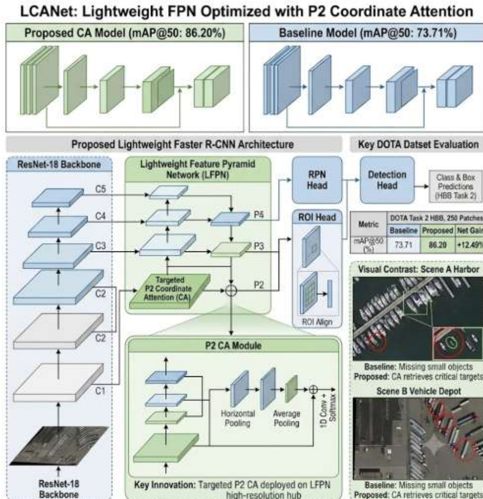
Figure 1. Overall architecture of the proposed framework (lcanet). Data flows from the resnet-18 backbone through the lightweight fpn; the p2 coordinate attention (ca) module enforces directional and spatial anchoring at the highest-resolution level, recovering minute objects missed by the baseline and lifting performance to 86.20% Map@50.
