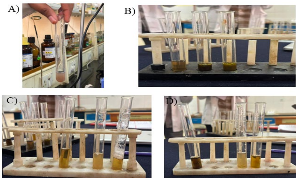
Figure 3: Phytochemical analysis of the fortified formulation showing the qualitative and quantitative presence of bioactive compounds contributing to its nutritional and functional properties.
