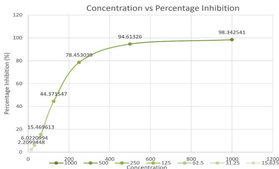
Figure 9: The graphical representation illustrates the scavenging kinetics of the fortified soup mix, showcasing a characteristic hyperbolic curve
